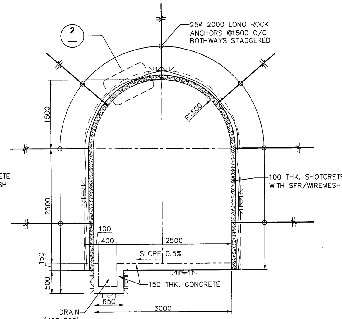
ROCK SUPPORT (CLASS-IV / VA)
