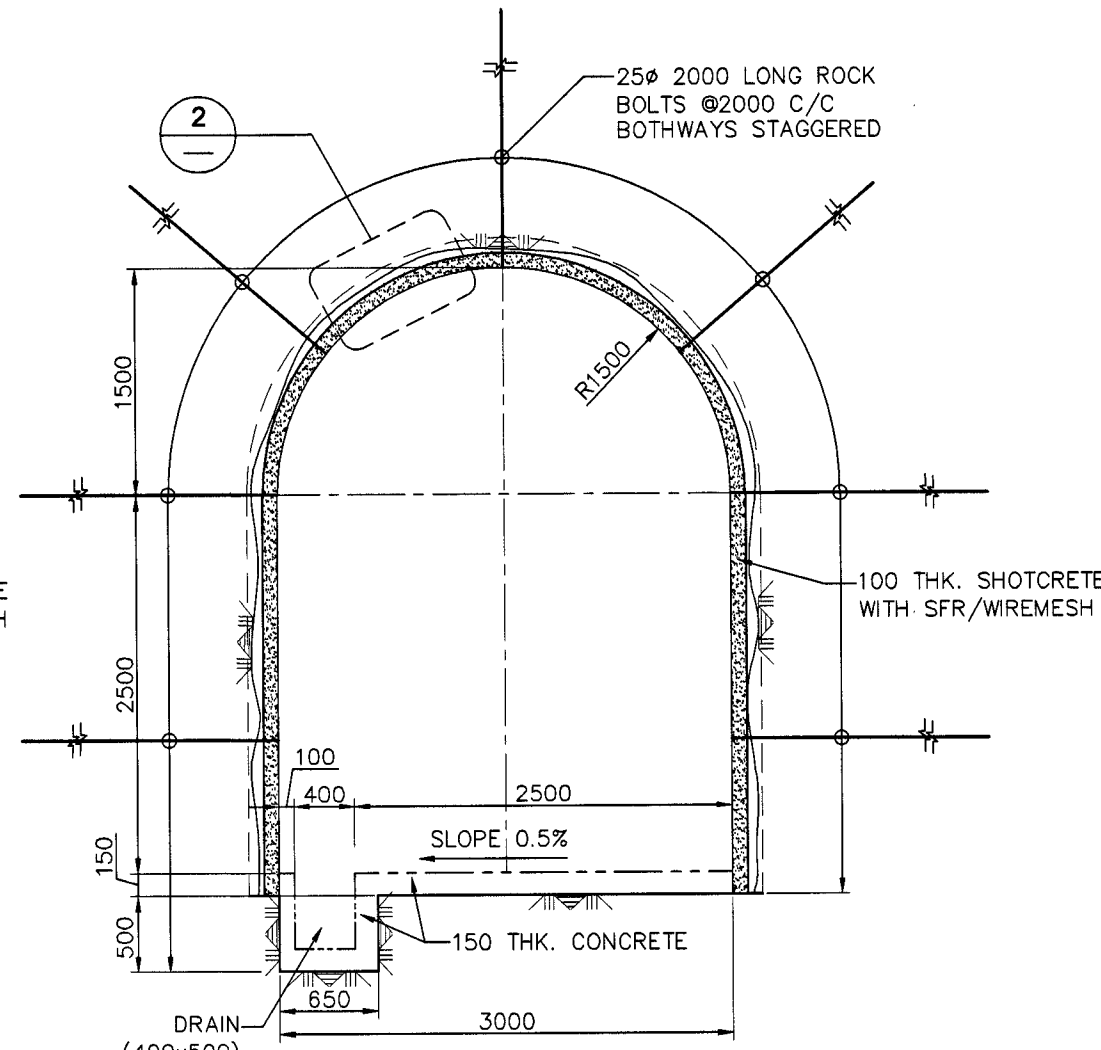
ROCK SUPPORT (CLASS-III)
