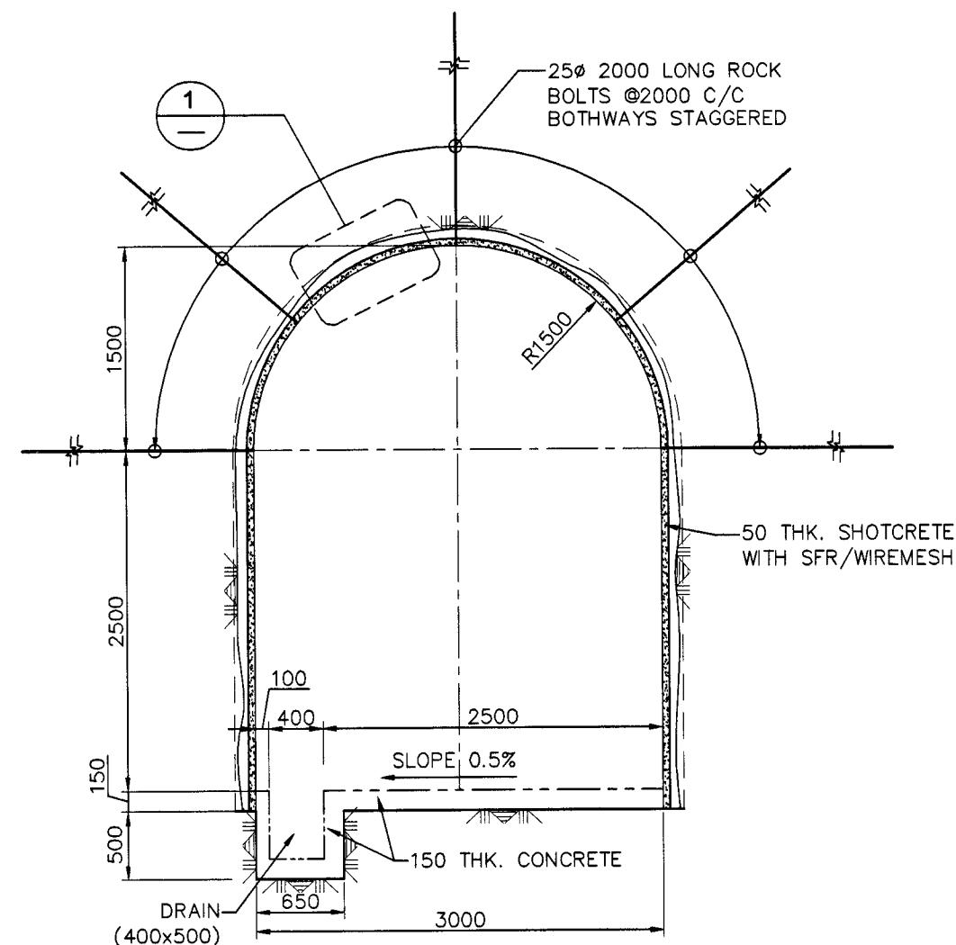
ROCK SUPPORT (CLASS-II)
